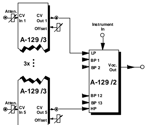
Fig. 5: A-129 /2 and A-129 /3s as a filter bank
